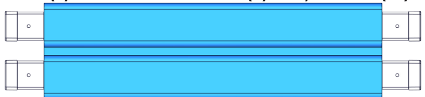
P2 - (1) 108" Canvas Roof with (2) 50 1/2" 2x4's (x1)
